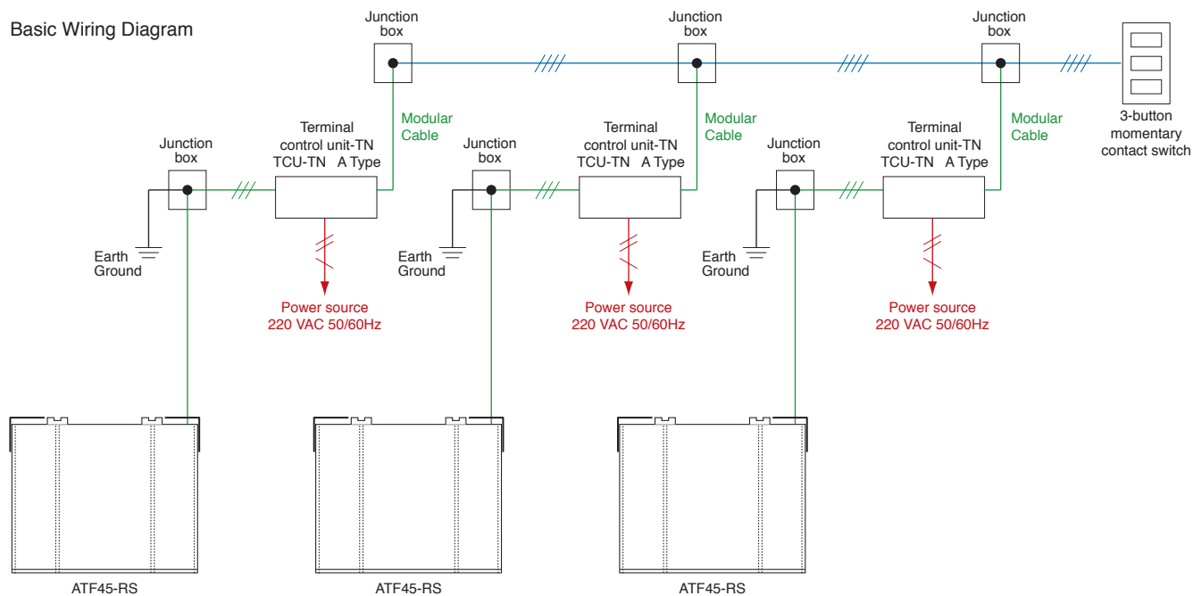
Basic Connecting Diagram
