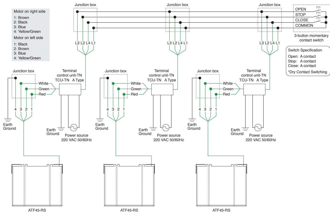
Basic Connecting Diagram
