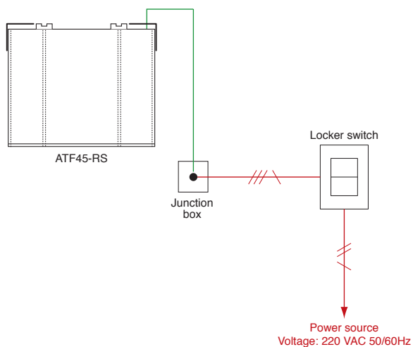
Basic Wiring Diagram
