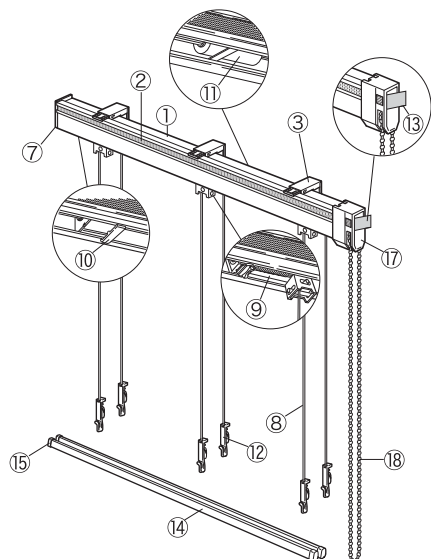
Drum type twin one chain
