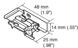
Ceiling Bracket
