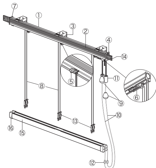
One-sided operation
