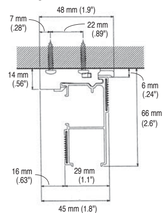
Ceiling attachment (With Ceiling Bracket)
