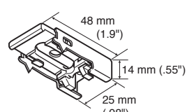
Ceiling Bracket
