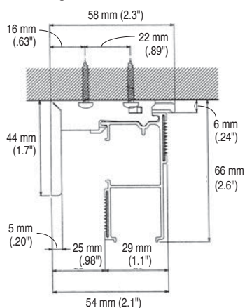
Ceiling attachment (With Universal Bracket)
