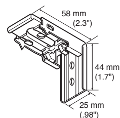
Universal Bracket
