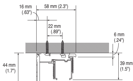
Ceiling attachment (With Universal Bracket)
