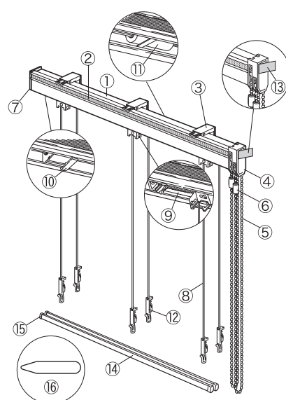
One-sided operation
