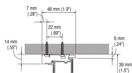
Ceiling attachment (With Ceiling Bracket)
