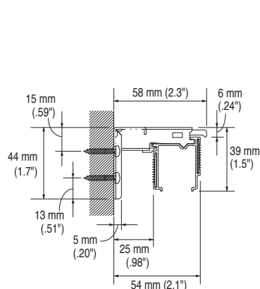
Wall attachment (With Universal Bracket)
