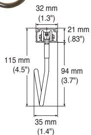
IV Roller Dimensions
