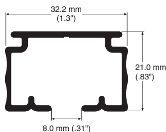
Rail Cross Section
