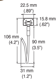
IV Roller Dimensions
