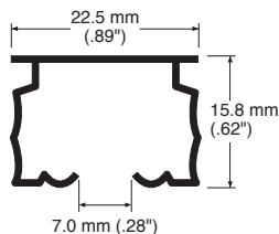
Rail Cross Section
